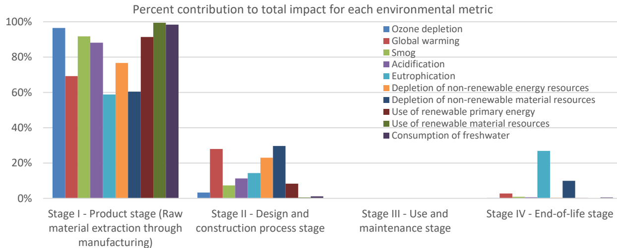
Figure 3 - Graphical impacts for the average Speedhide Interior Latex product showing % contribution by life cycle stage
